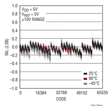
LTC2755-16 Integral Nonlinearity (INL)
