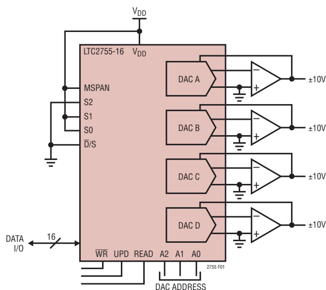
Figure 1. Using MSPAN to Configure the LTC2755 for Single-Span Operation ( \pm 10\text{V} Range).
