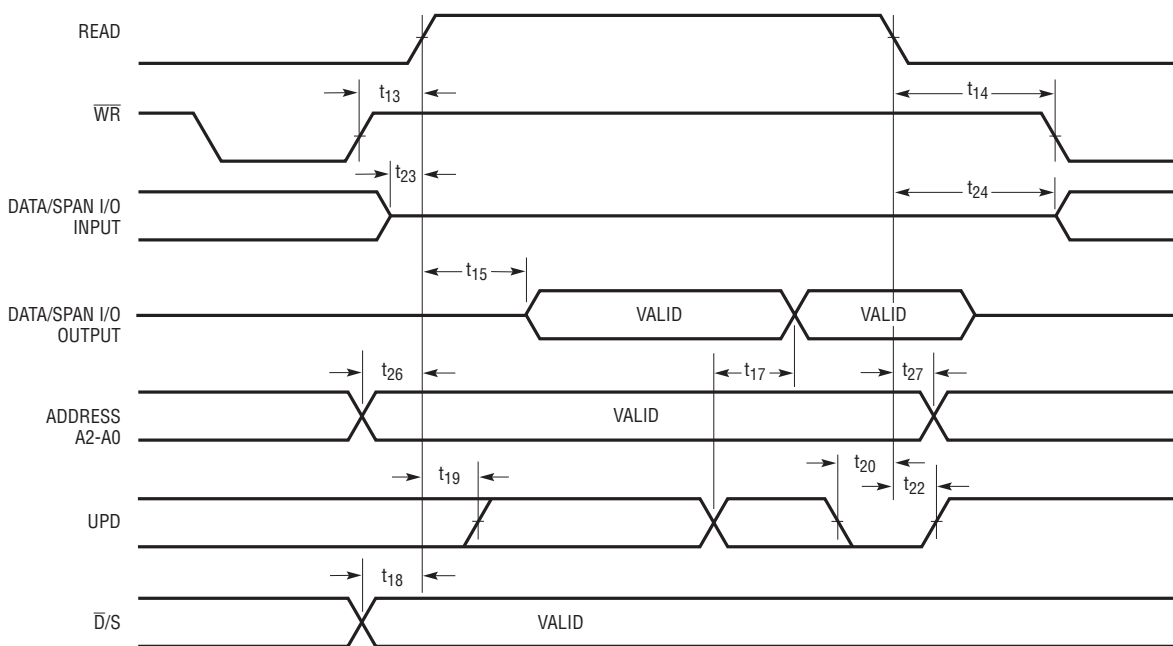
Readback Timing
